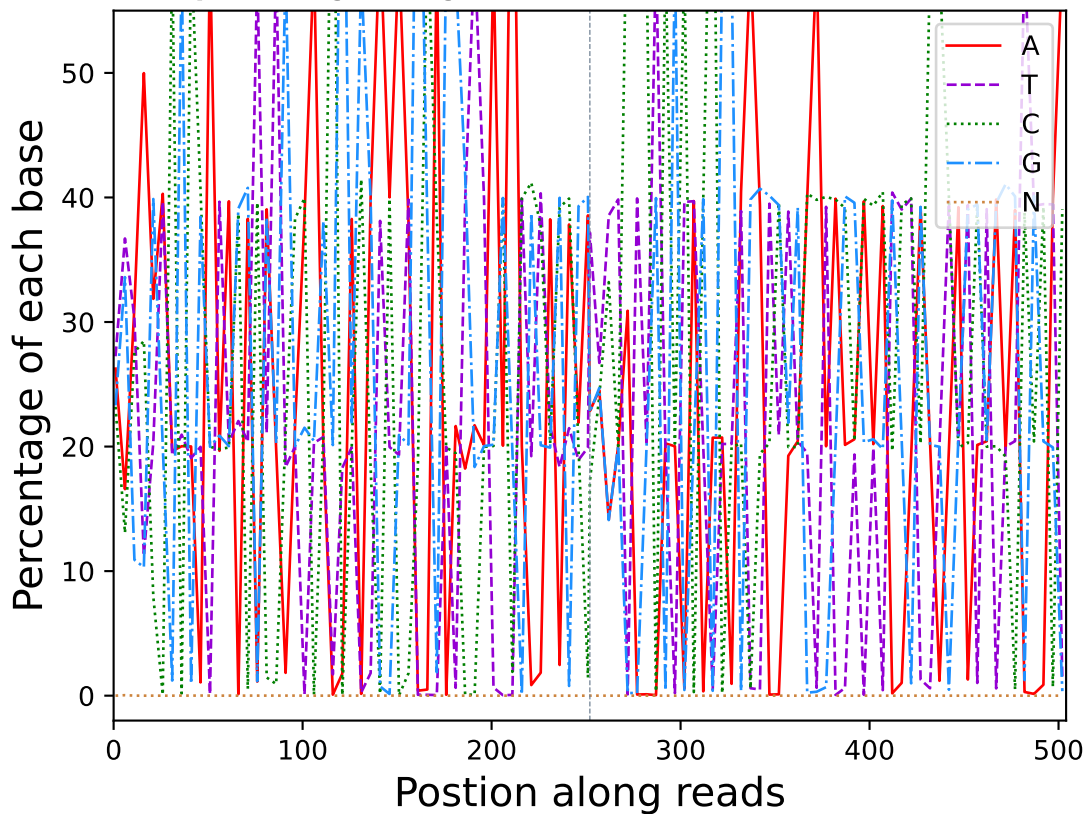
Base percentage along reads (R20114)
